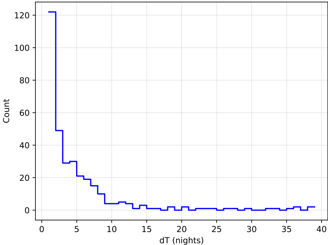
too_elab_r32_d2_griz_v3.4_10yrs all bands: DD:WFD Delta Nights Histogram
