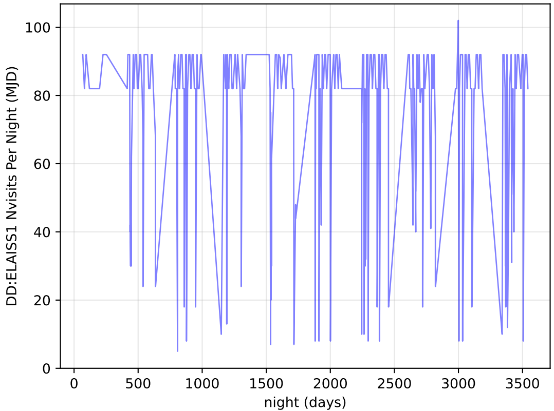
too_elab_r32_d2_griz_v3.4_10yrs all bands: DD:ELAISS1 Nvisits Per Night
