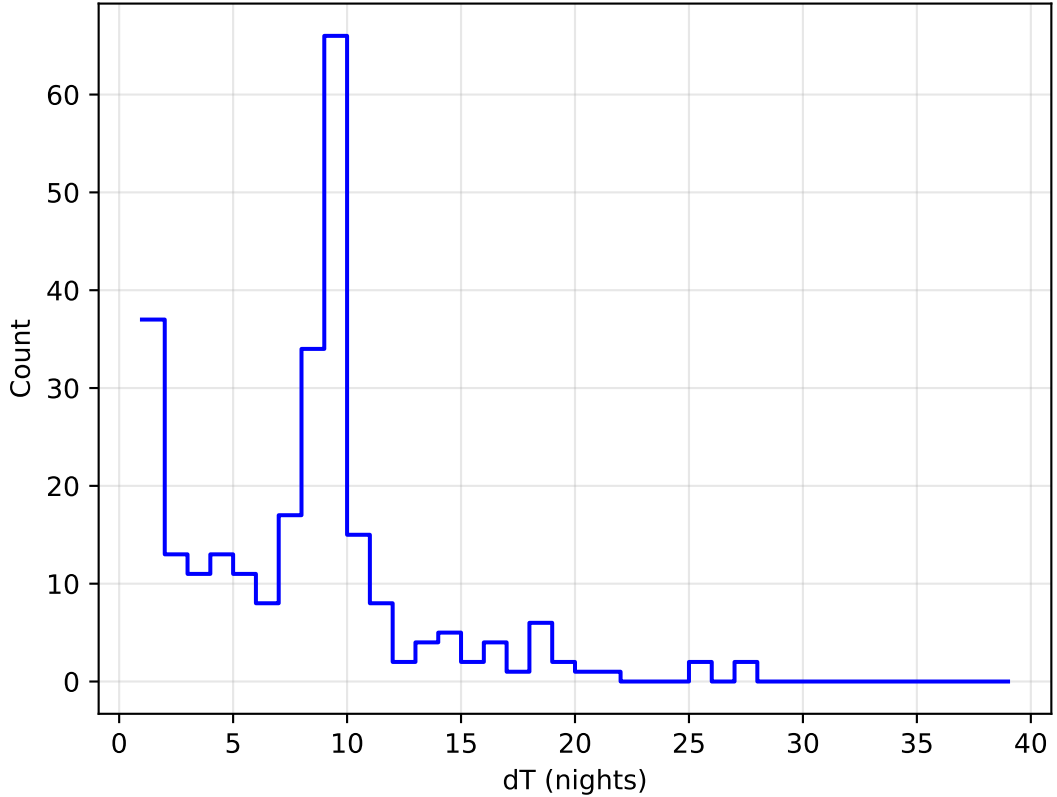
too_elab_r32_d2_griz_v3.4_10yrs all bands: DD:ELAISS1 Delta Nights Histogram
