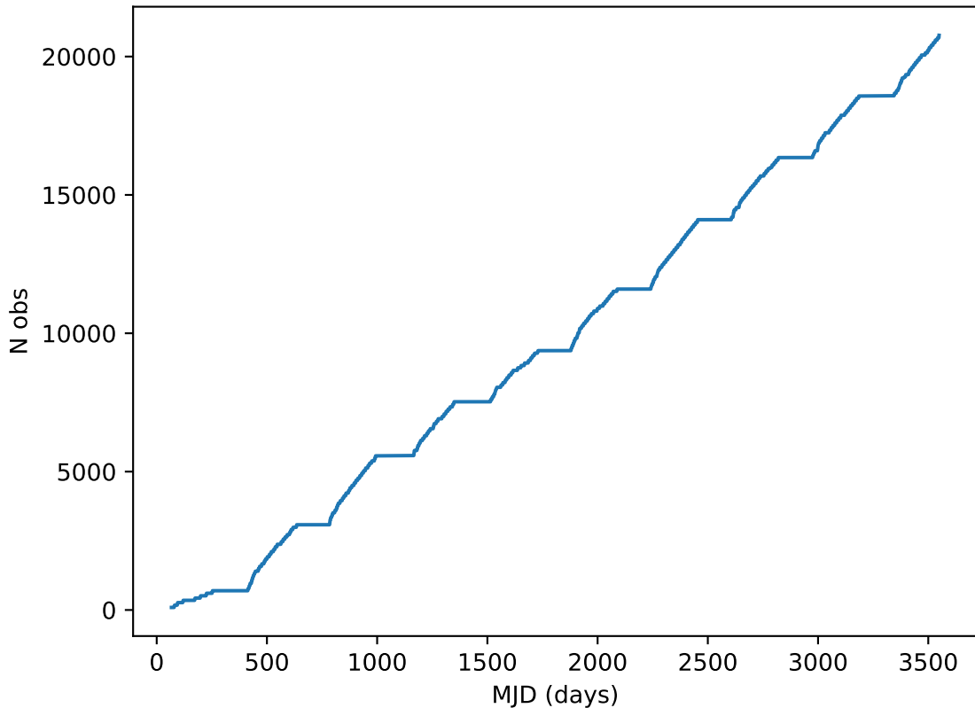
too_elab_r32_d2_griz_v3.4_10yrs all bands: DD:ELAISS1 Cumulative NVisits
