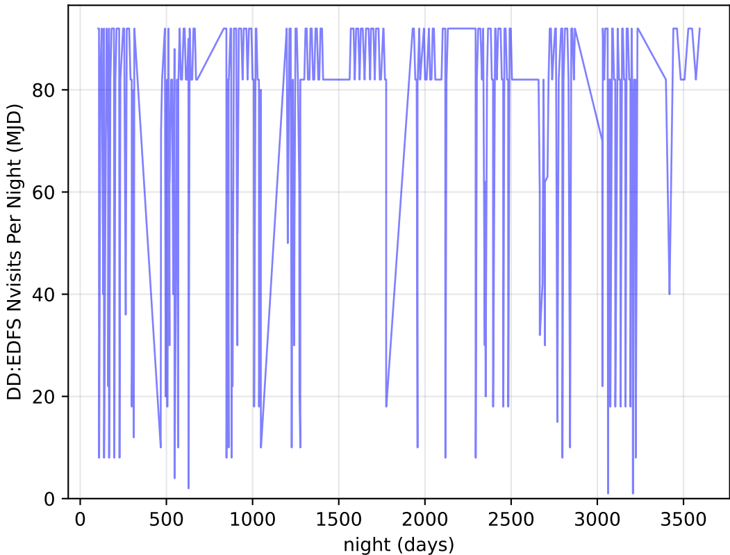
too_elab_r32_d2_griz_v3.4_10yrs all bands: DD:EDFS Nvisits Per Night
