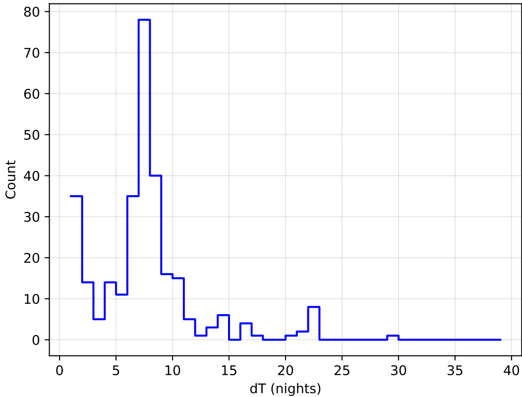
too_elab_r32_d2_griz_v3.4_10yrs all bands: DD:EDFS Delta Nights Histogram
