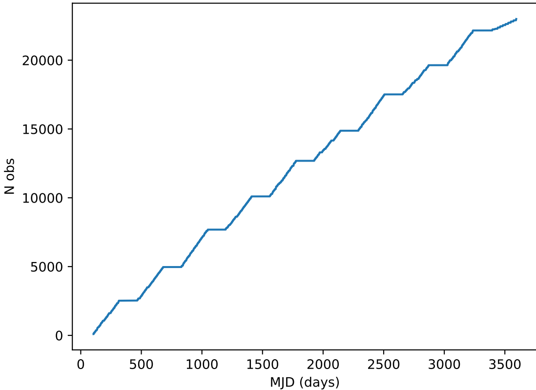
too_elab_r32_d2_griz_v3.4_10yrs all bands: DD:EDFS Cumulative NVisits
