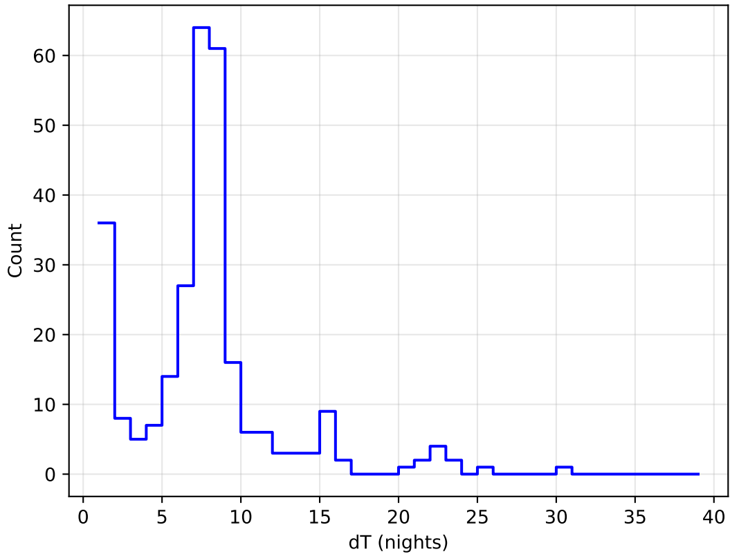
too_elab_r32_d2_griz_v3.4_10yrs all bands: DD:ECDFS Delta Nights Histogram
