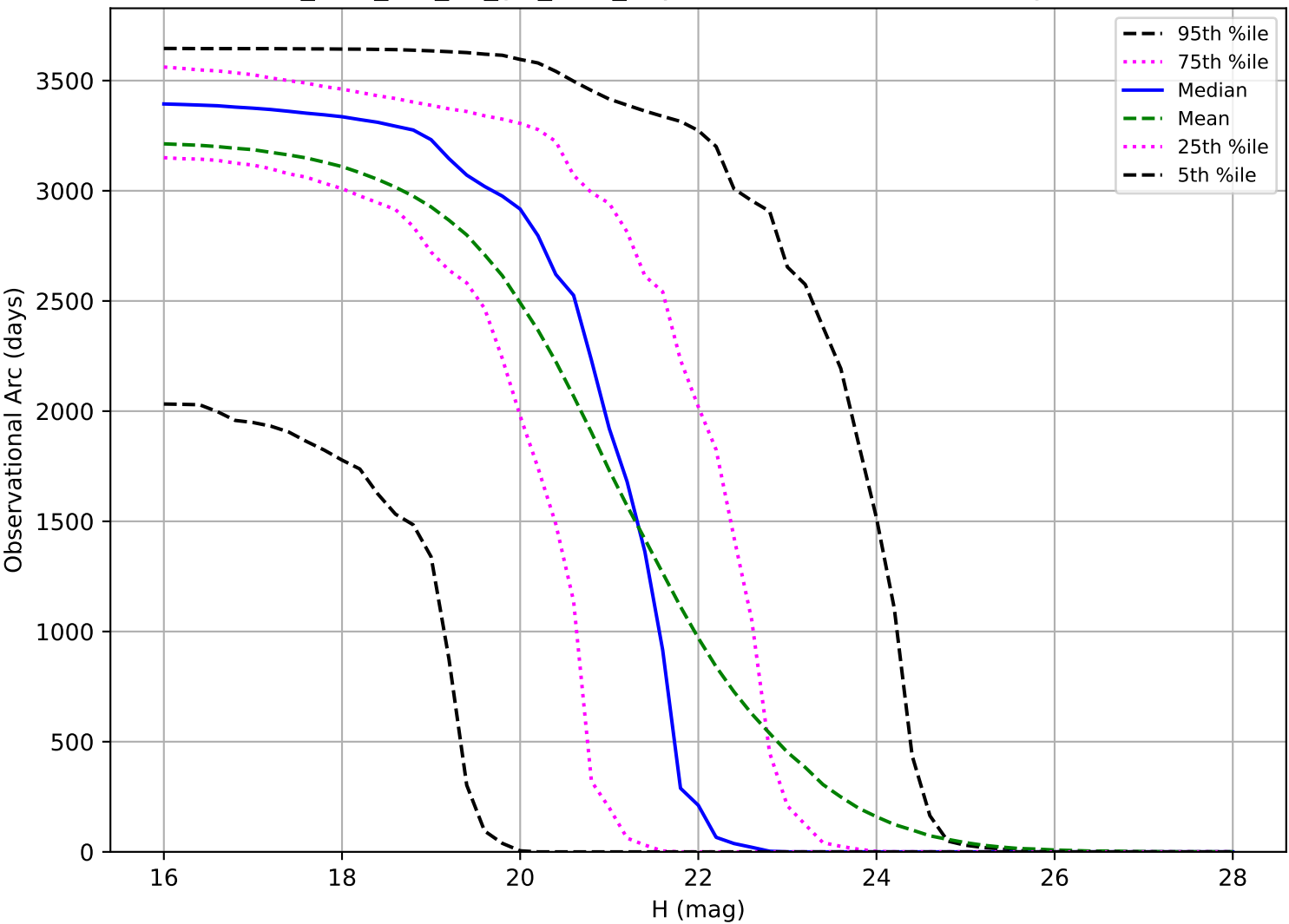
too_elab_r32_d2_giz_v3.4_10yrs: Observational Arc Length PHA
