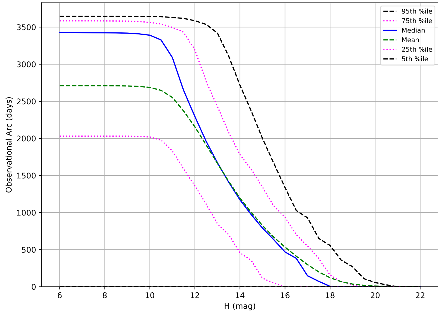
too_elab_r32_d2_giz_v3.4_10yrs: Observational Arc Length OCC_r5
