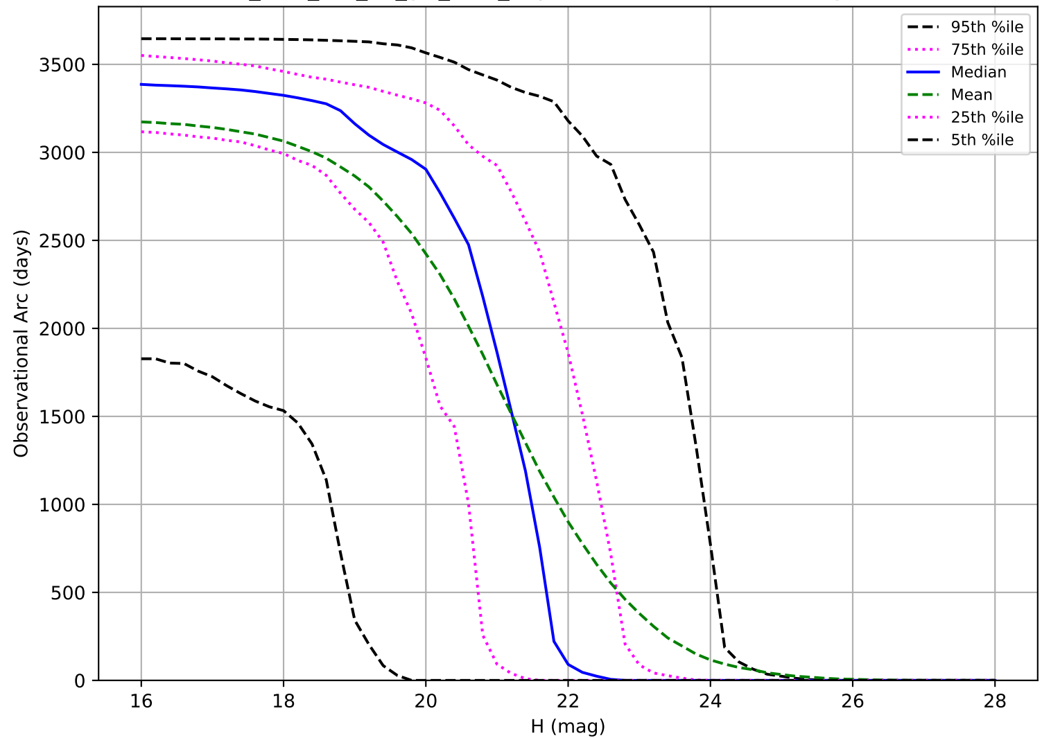
too_elab_r32_d2_giz_v3.4_10yrs: Observational Arc Length NEO
