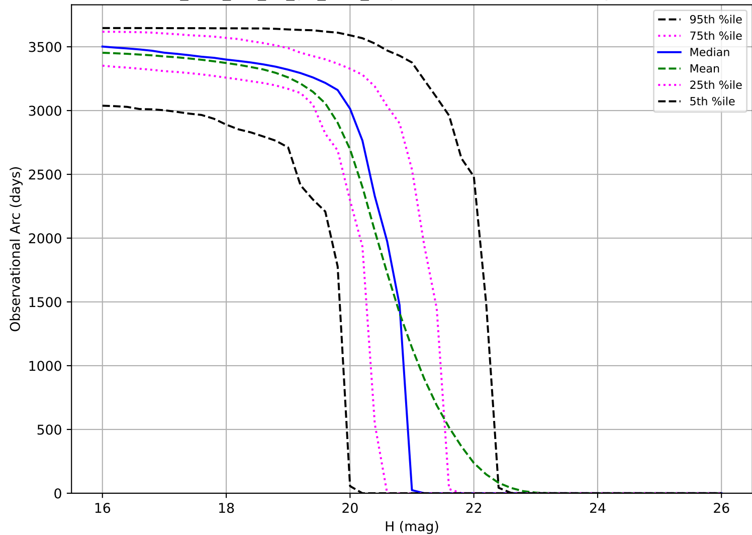
too_elab_r32_d2_giz_v3.4_10yrs: Observational Arc Length MBA
