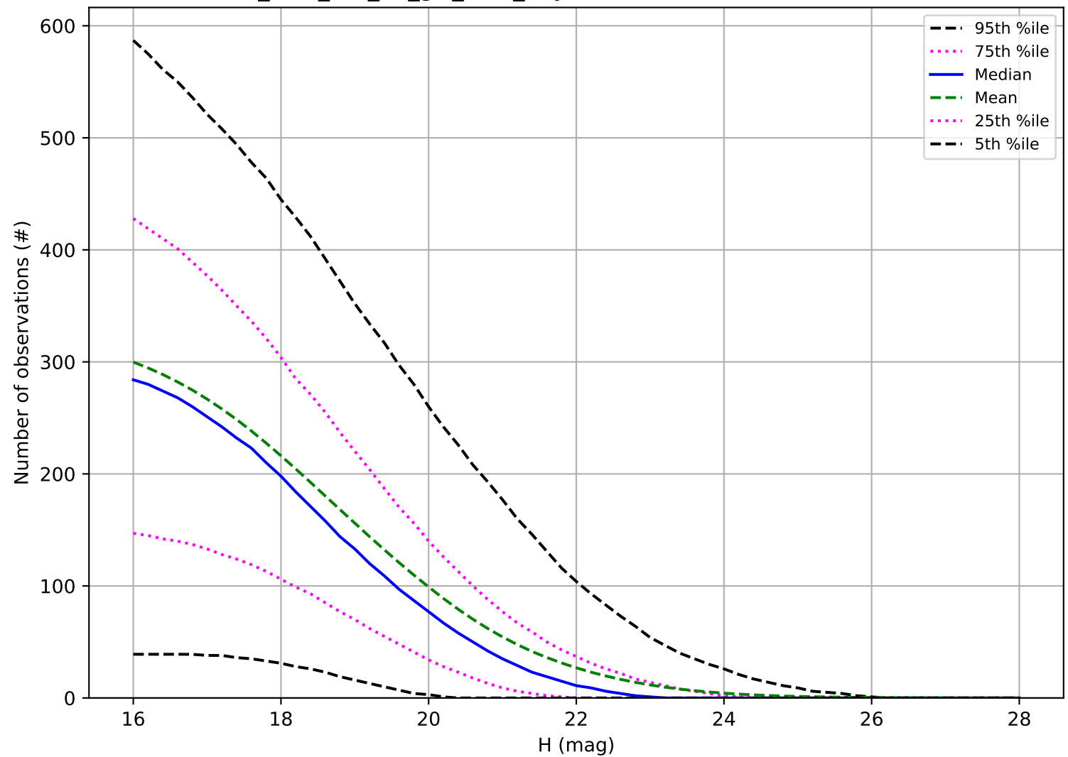
too_elab_r32_d2_giz_v3.4_10yrs: Number of observations PHA
