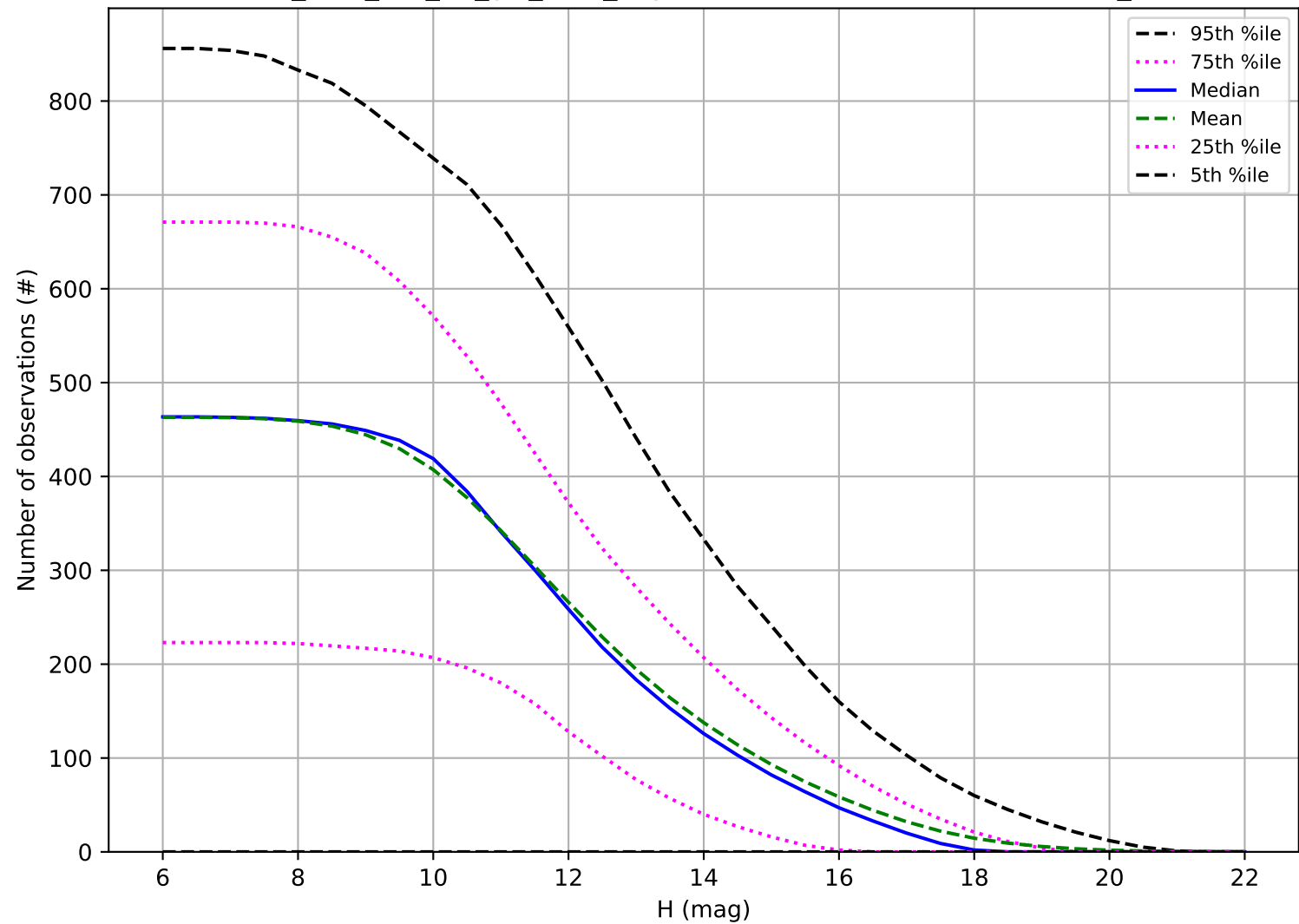
too_elab_r32_d2_giz_v3.4_10yrs: Number of observations OCC_r5
