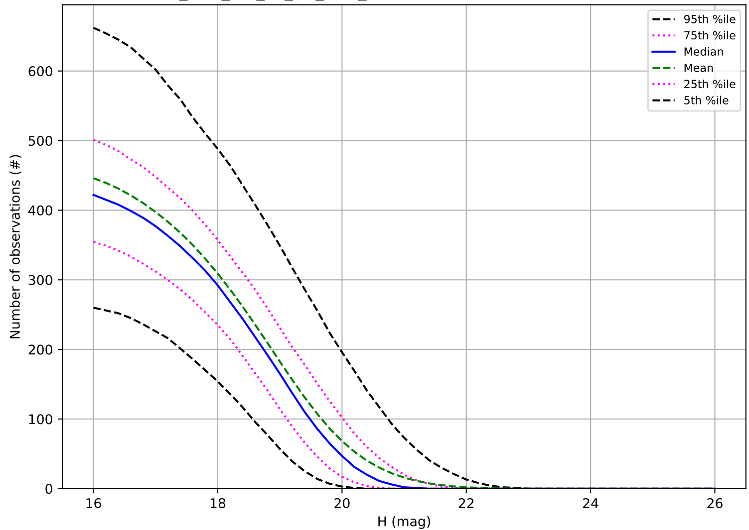
too_elab_r32_d2_giz_v3.4_10yrs: Number of observations MBA
