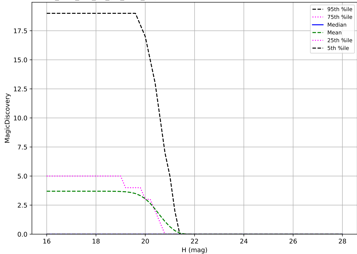
too_elab_r32_d2_giz_v3.4_10yrs: Vatira 6 detections in 60 nights detection loss
