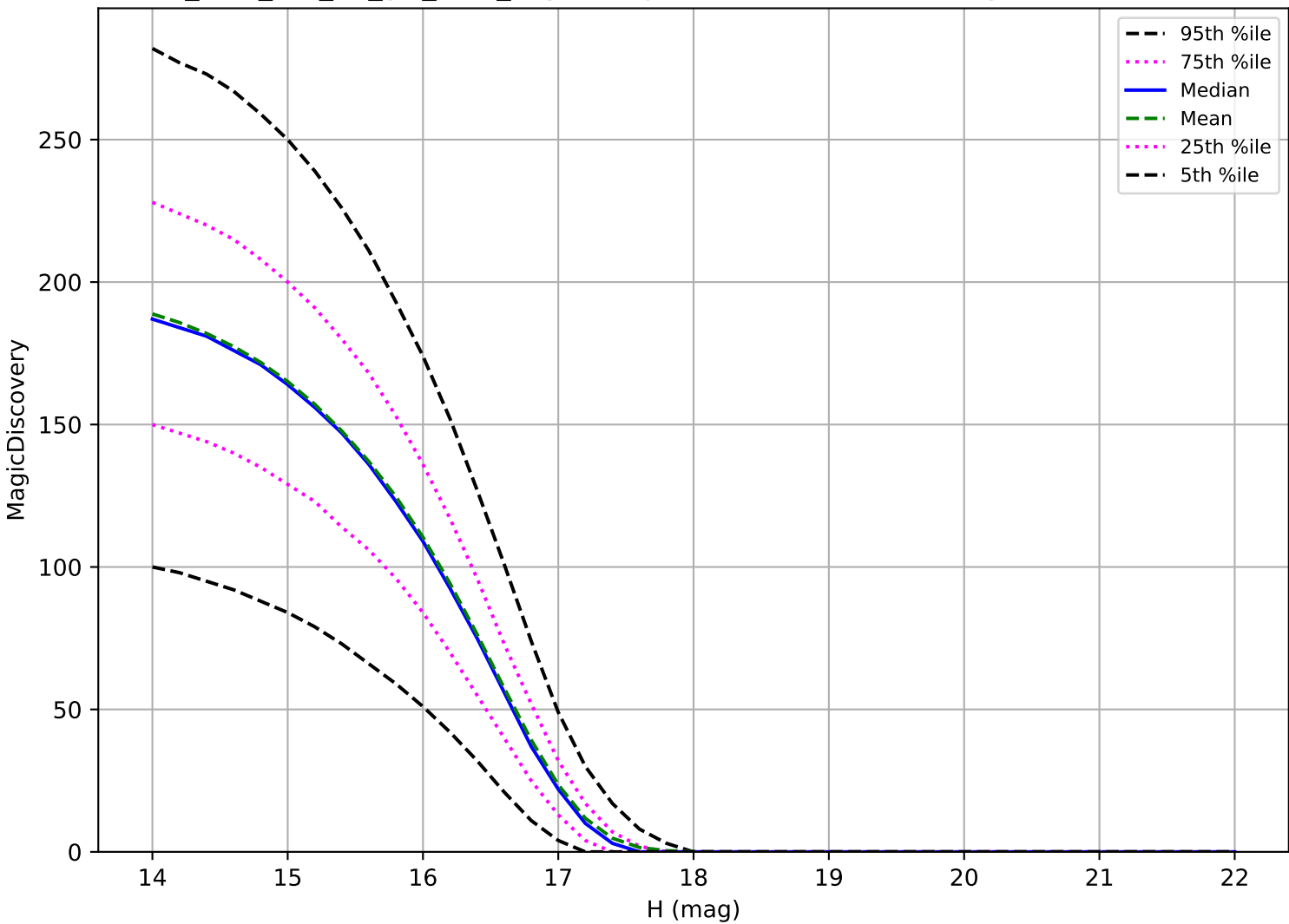
too_elab_r32_d2_giz_v3.4_10yrs: Trojan 6 detections in 60 nights detection loss
