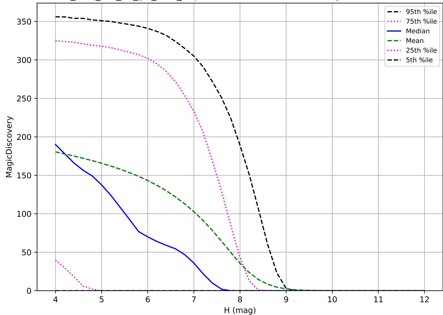
too_elab_r32_d2_giz_v3.4_10yrs: TNO 6 detections in 60 nights detection loss
