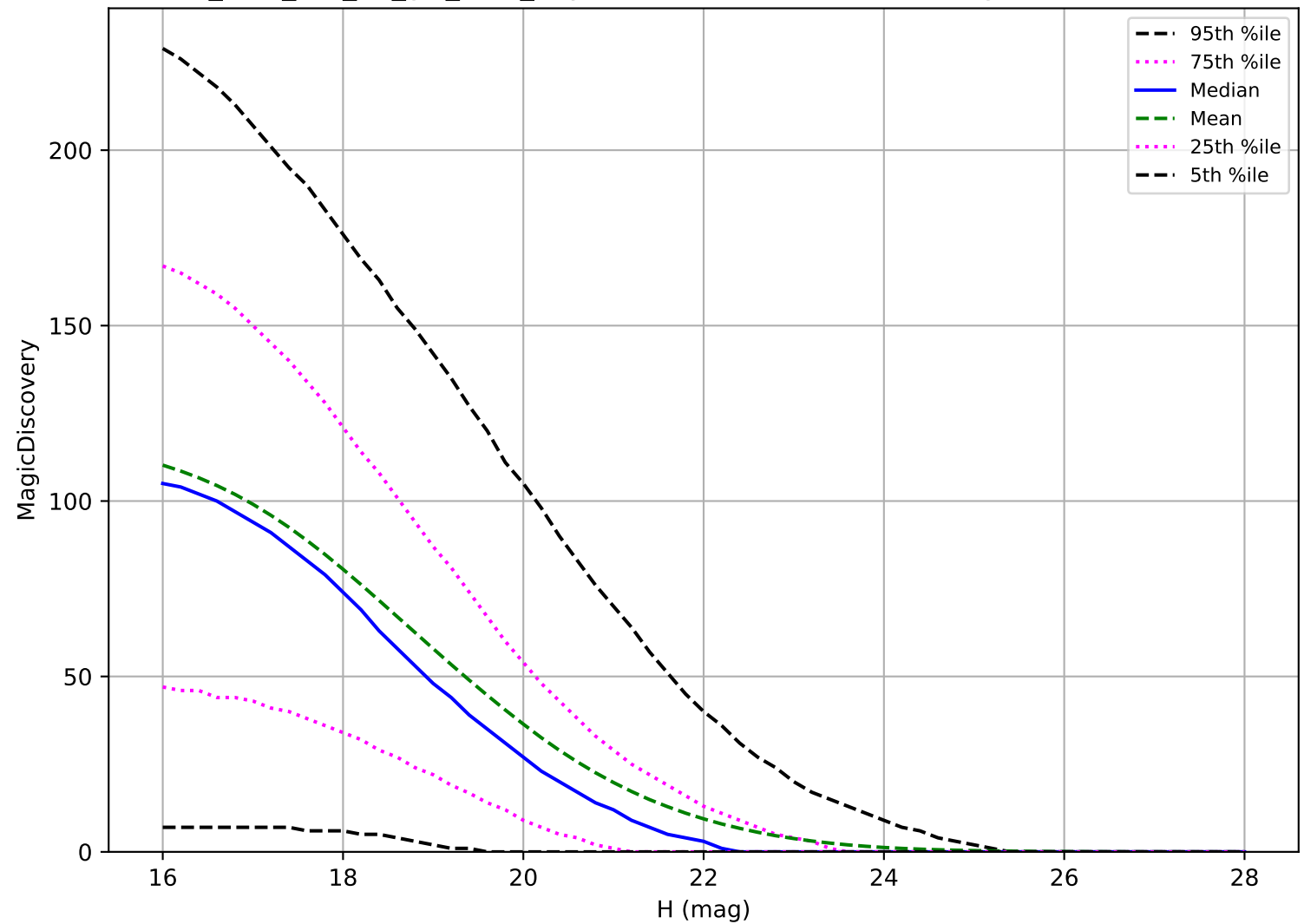
too_elab_r32_d2_giz_v3.4_10yrs: PHA 6 detections in 60 nights detection loss
