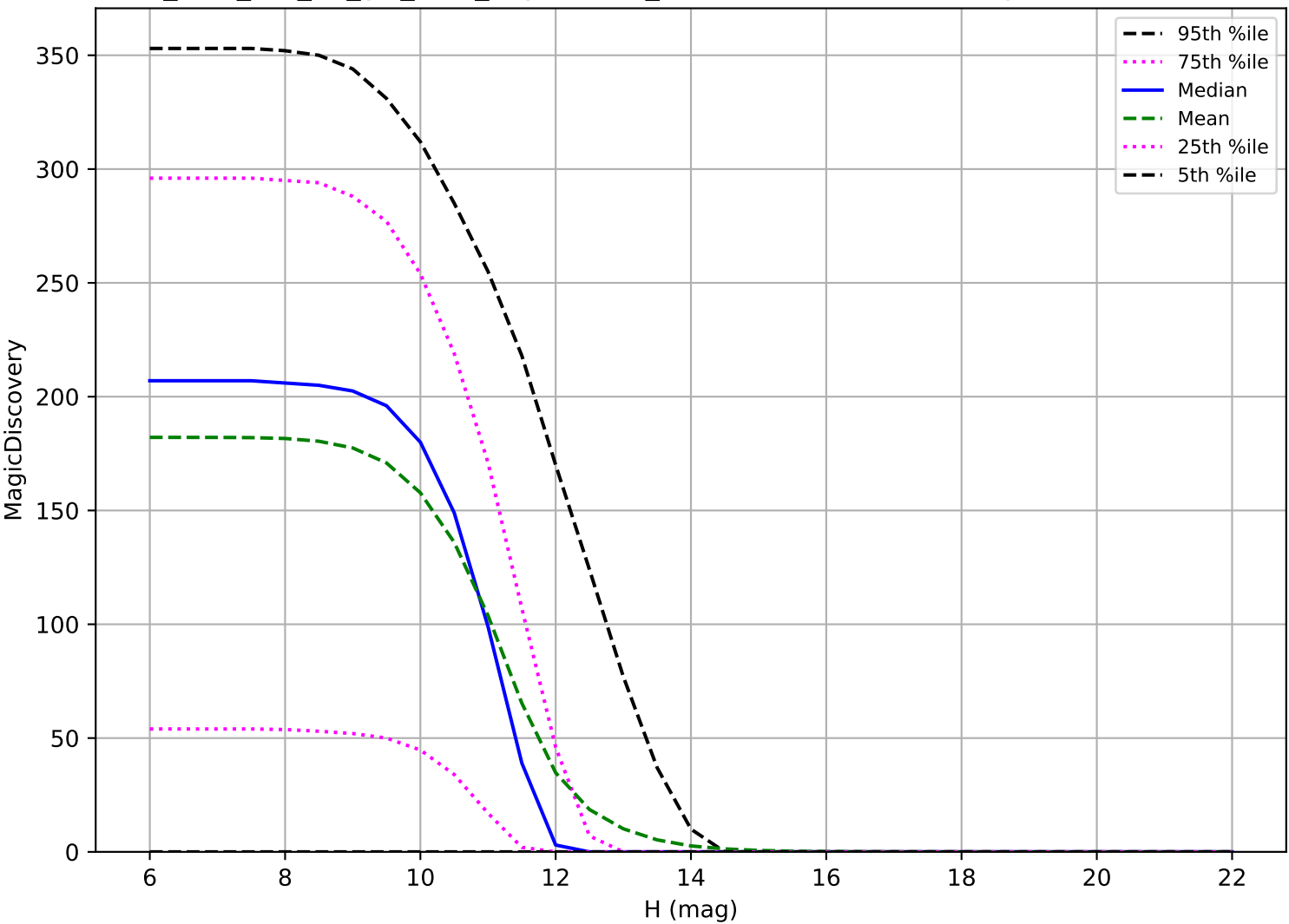
too_elab_r32_d2_giz_v3.4_10yrs: OCC_r20 6 detections in 60 nights detection loss
