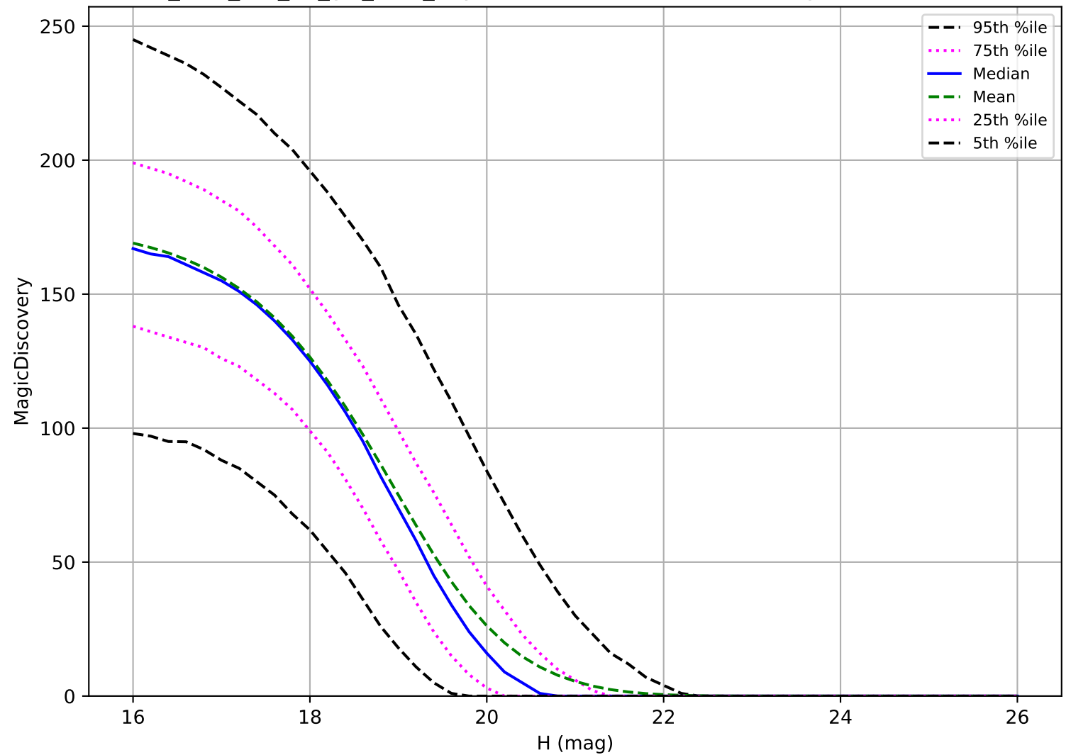
too_elab_r32_d2_giz_v3.4_10yrs: MBA 6 detections in 60 nights detection loss
