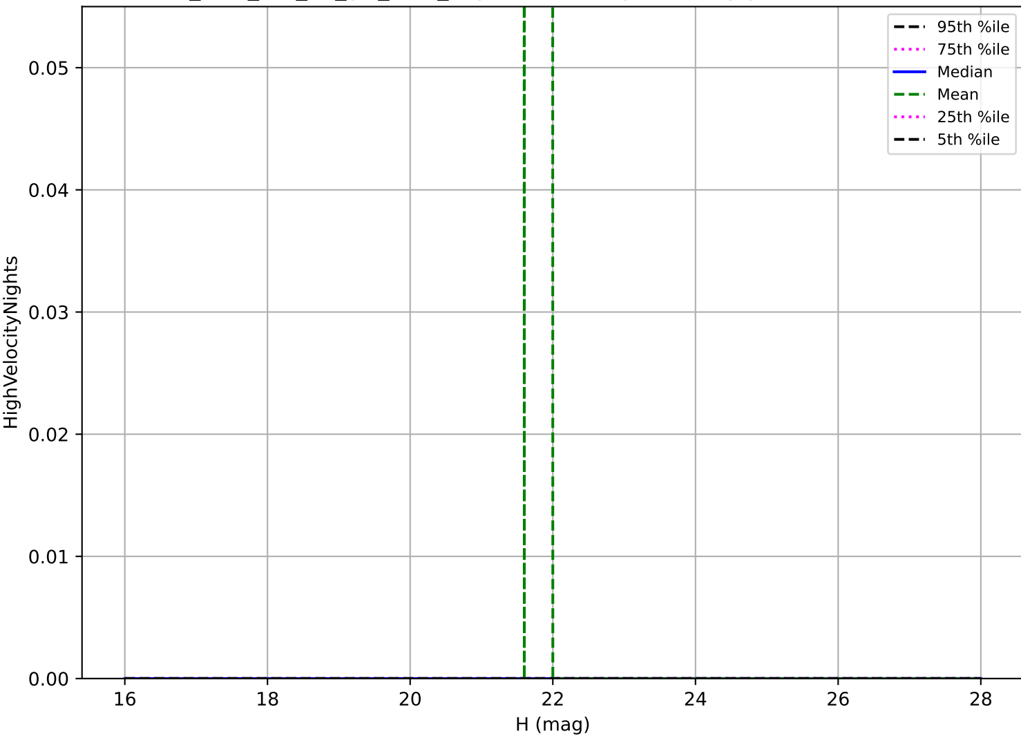
too_elab_r32_d2_giz_v3.4_10yrs: Vatra High velocity pair detection loss
