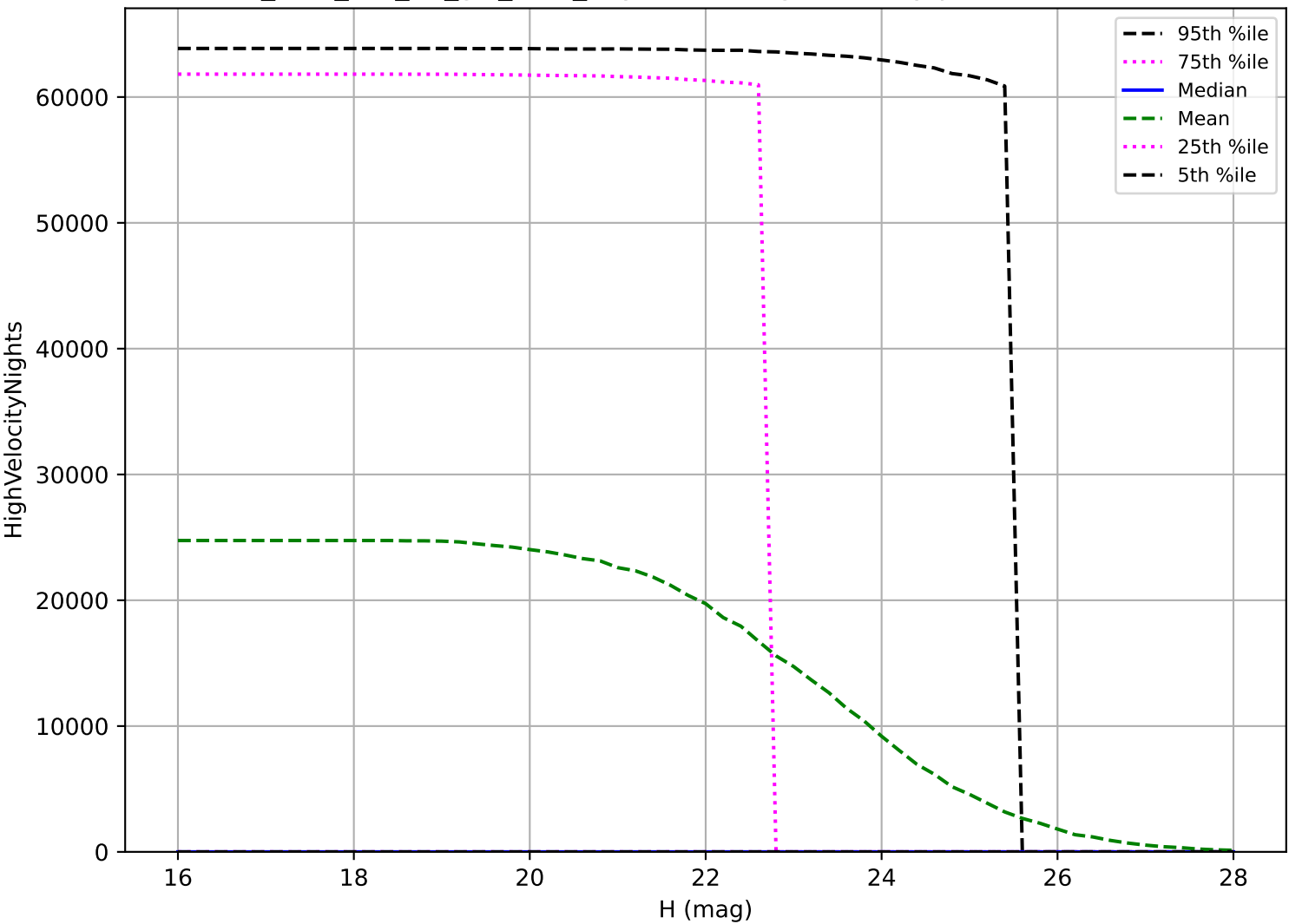
too_elab_r32_d2_giz_v3.4_10yrs: PHA High velocity pair detection loss
