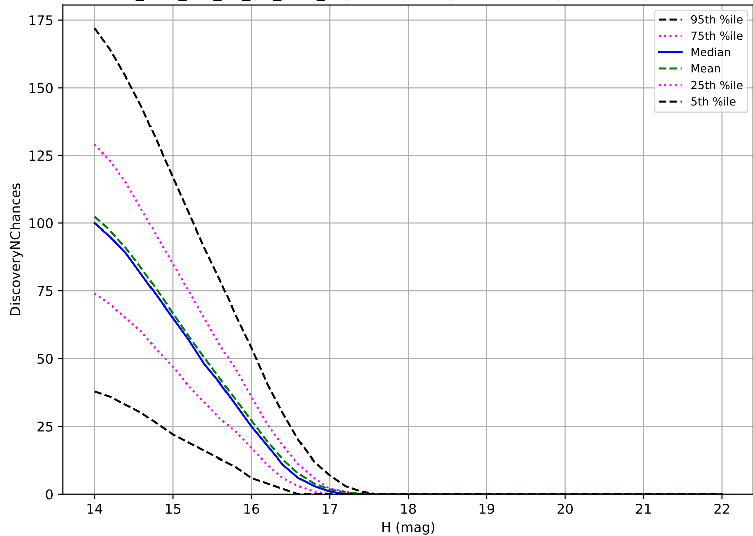
too_elab_r32_d2_giz_v3.4_10yrs: Trojan 3 pairs in 15 nights detection loss
