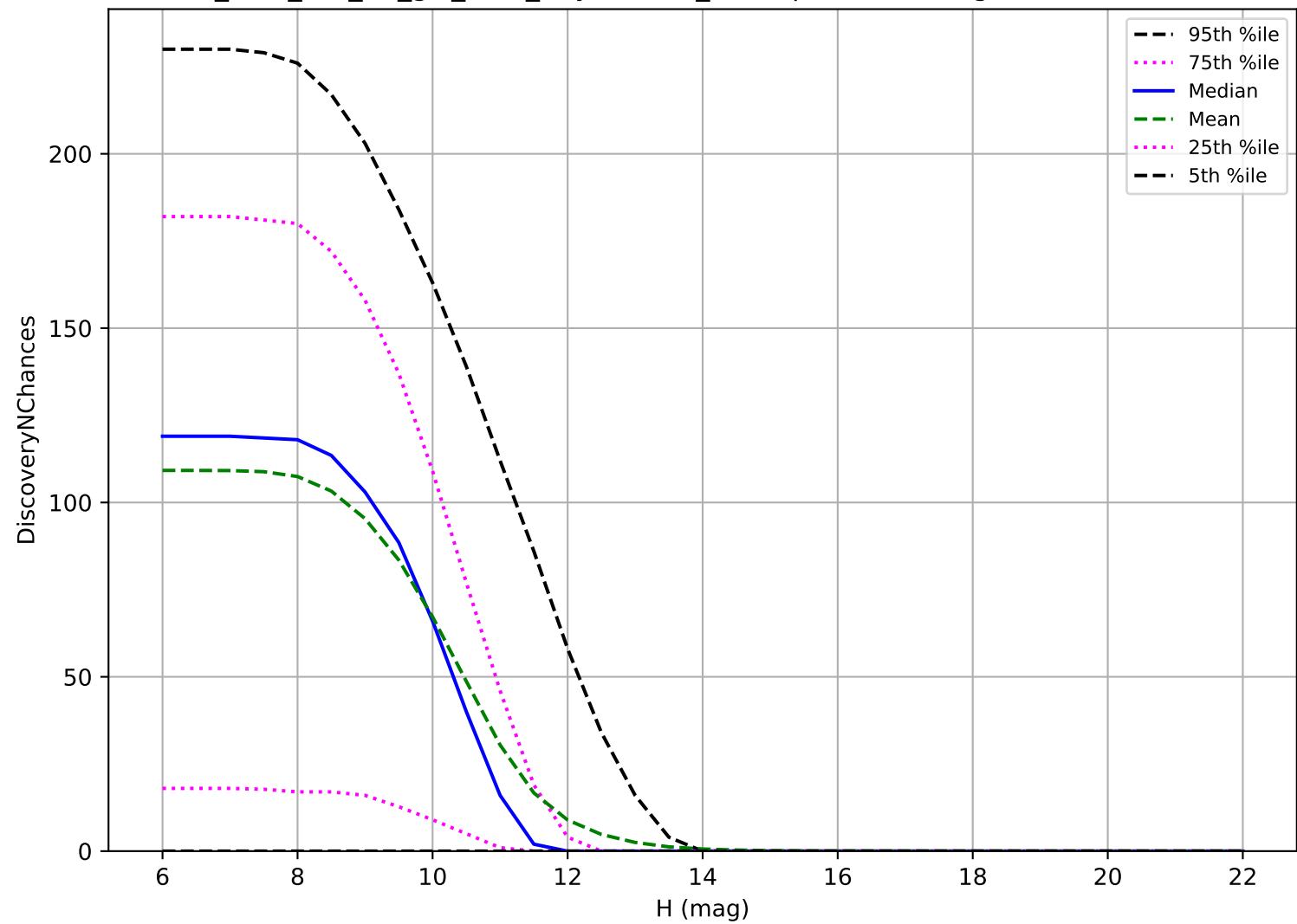
too_elab_r32_d2_giz_v3.4_10yrs: OCC_r20 3 pairs in 15 nights detection loss
