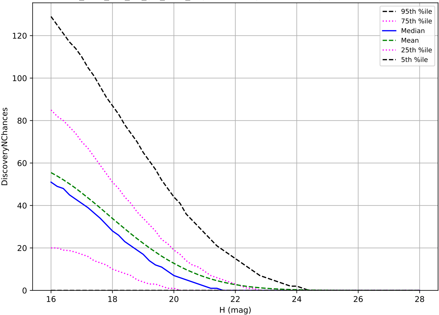
too_elab_r32_d2_giz_v3.4_10yrs: NEO 3 pairs in 15 nights detection loss
