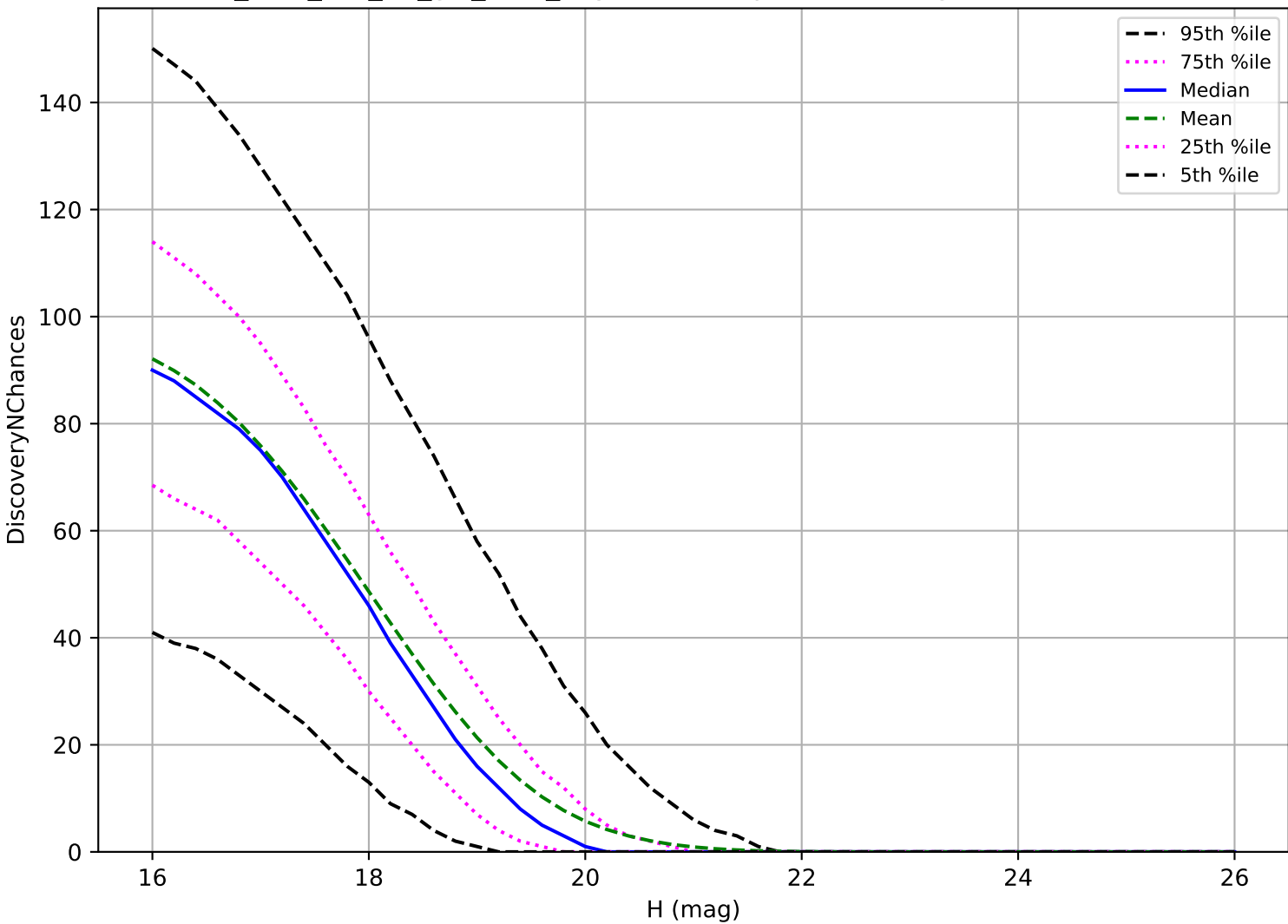
too_elab_r32_d2_giz_v3.4_10yrs: MBA 3 pairs in 15 nights detection loss
