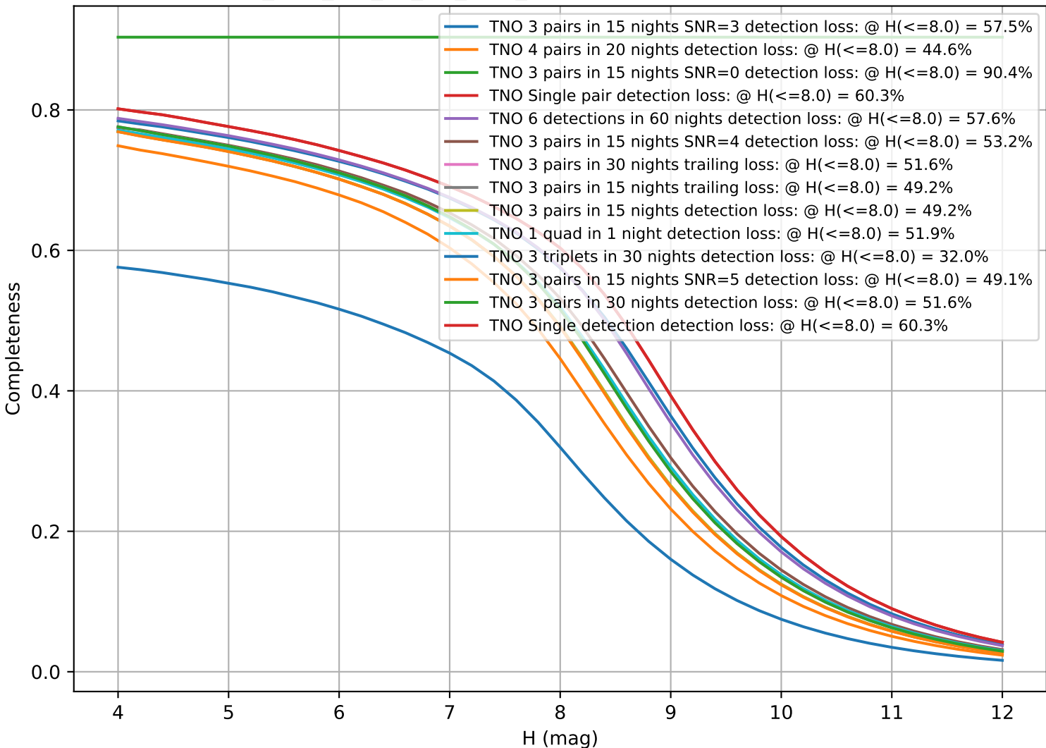
too_elab_r32_d2_giz_v3.4_10yrs: CumulativeCompleteness
