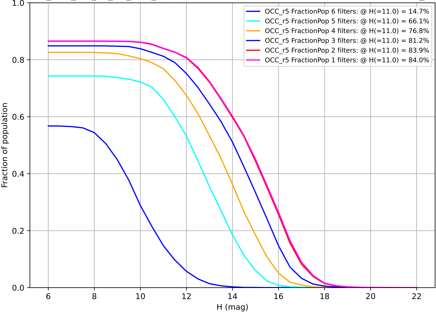
too_elab_r32_d2_giz_v3.4_10yrs: Fraction of population with colors in X filters OCC_r5
