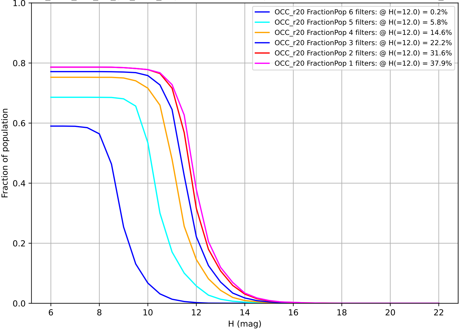
too_elab_r32_d2_giz_v3.4_10yrs: Fraction of population with colors in X filters OCC_r20
