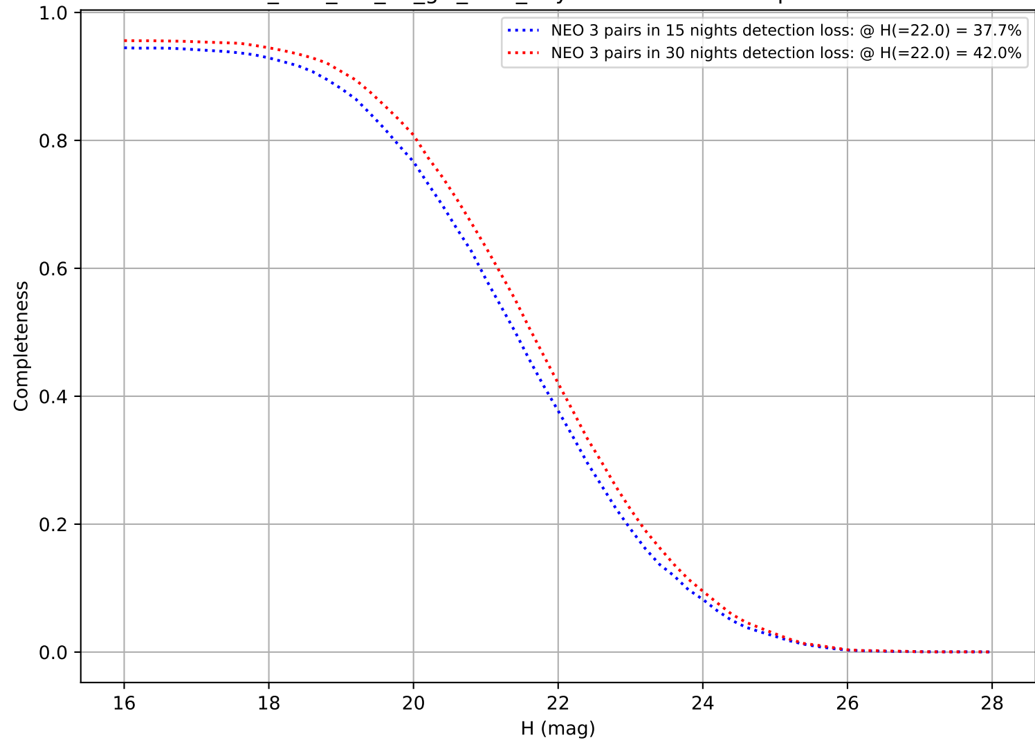
too_elab_r32_d2_giz_v3.4_10yrs: DifferentialCompleteness
