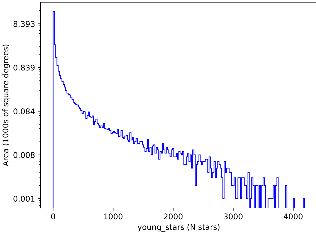
too_elab_r32_d2_giz_v3.4_10yrs : young_stars
