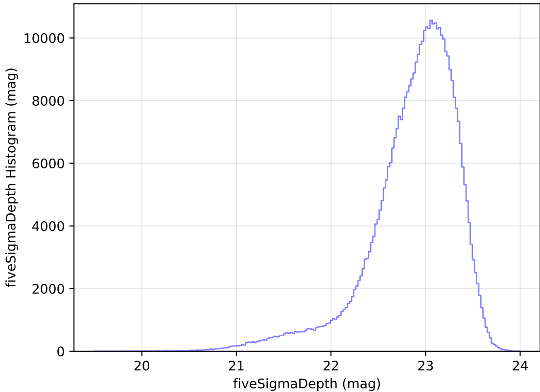
too_elab_r32_d2_giz_v3.4_10yrs z: fiveSigmaDepth Histogram
