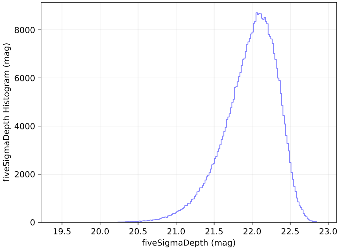
too_elab_r32_d2_giz_v3.4_10yrs y: fiveSigmaDepth Histogram
