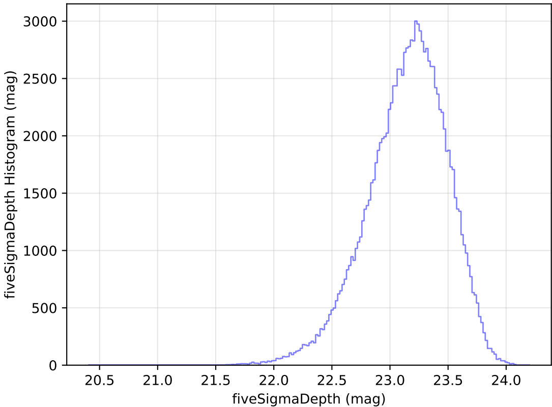
too_elab_r32_d2_giz_v3.4_10yrs u: fiveSigmaDepth Histogram
