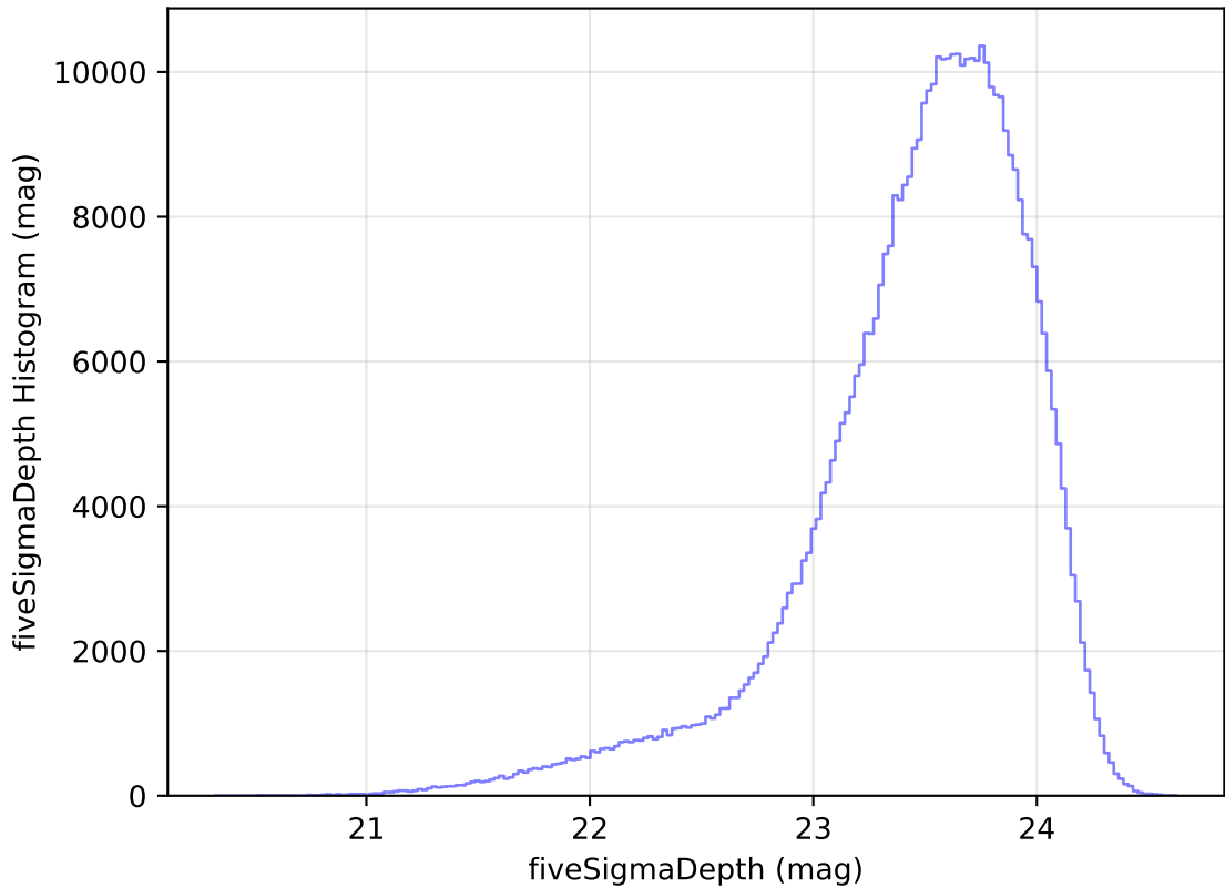
too_elab_r32_d2_giz_v3.4_10yrs i: fiveSigmaDepth Histogram
