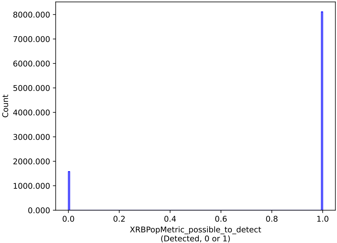
too_elab_r32_d2_giz_v3.4_10yrs : XRBPoMetric_possible_to_detect
