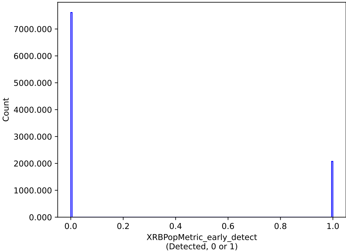
too_elab_r32_d2_giz_v3.4_10yrs : XRBPoMetric_early_detect
