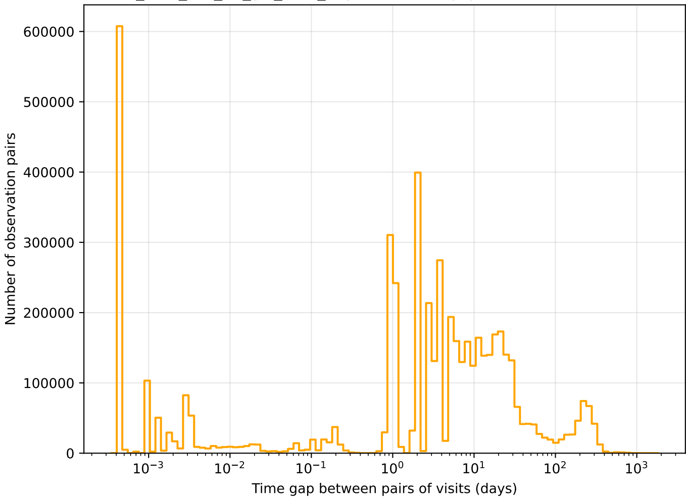
too_elab_r32_d2_giz_v3.4_10yrs r band: Tgaps observationStartMJD
