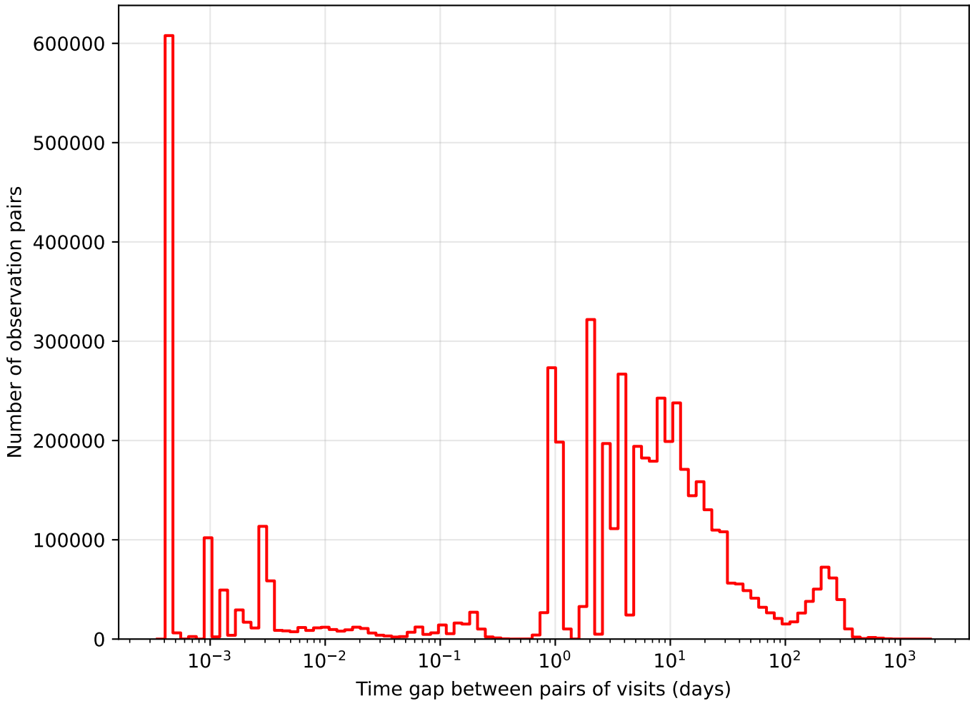
too_elab_r32_d2_giz_v3.4_10yrs i band: Tgaps observationStartMJD
