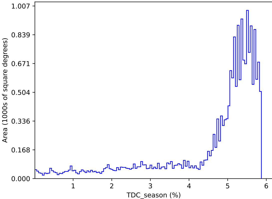
too_elab_r32_d2_giz_v3.4_10yrs : TDC_season
