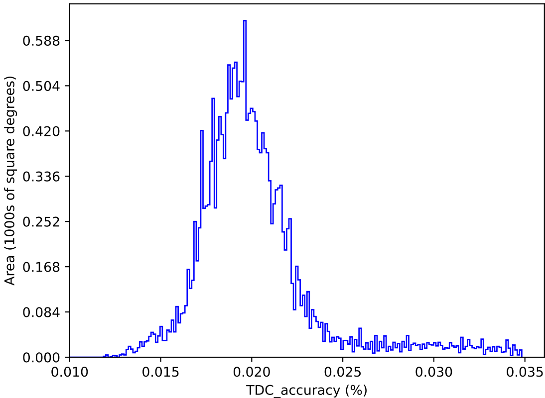
too_elab_r32_d2_giz_v3.4_10yrs : TDC_accuracy
