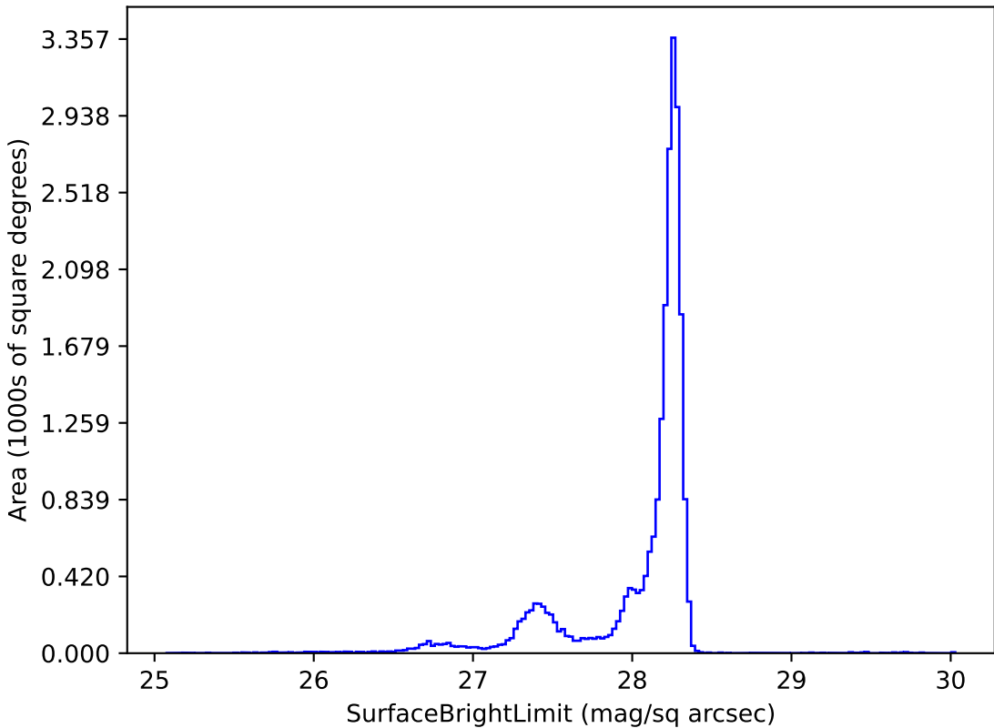
too_elab_r32_d2_giz_v3.4_10yrs y: SurfaceBrightLimit
