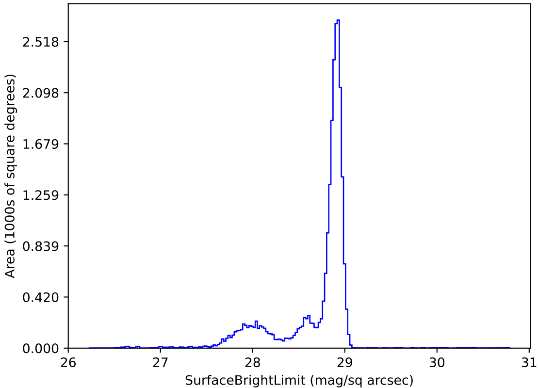
too_elab_r32_d2_giz_v3.4_10yrs u: SurfaceBrightLimit
