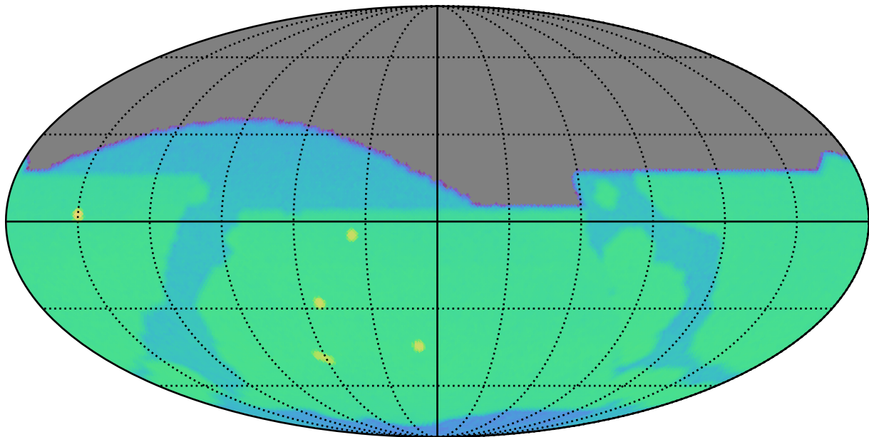
too_elab_r32_d2_giz_v3.4_10yrs r: SurfaceBrightLimit
