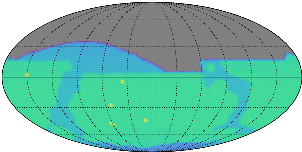
too_elab_r32_d2_giz_v3.4_10yrs i: SurfaceBrightLimit
