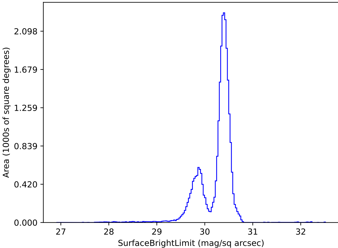
too_elab_r32_d2_giz_v3.4_10yrs g: SurfaceBrightLimit
