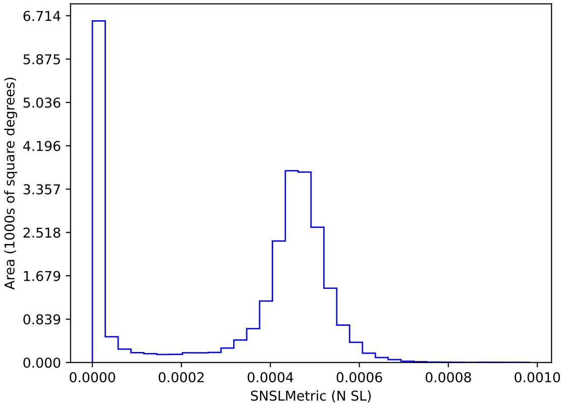
too_elab_r32_d2_giz_v3.4_10yrs : SNSLMetric
