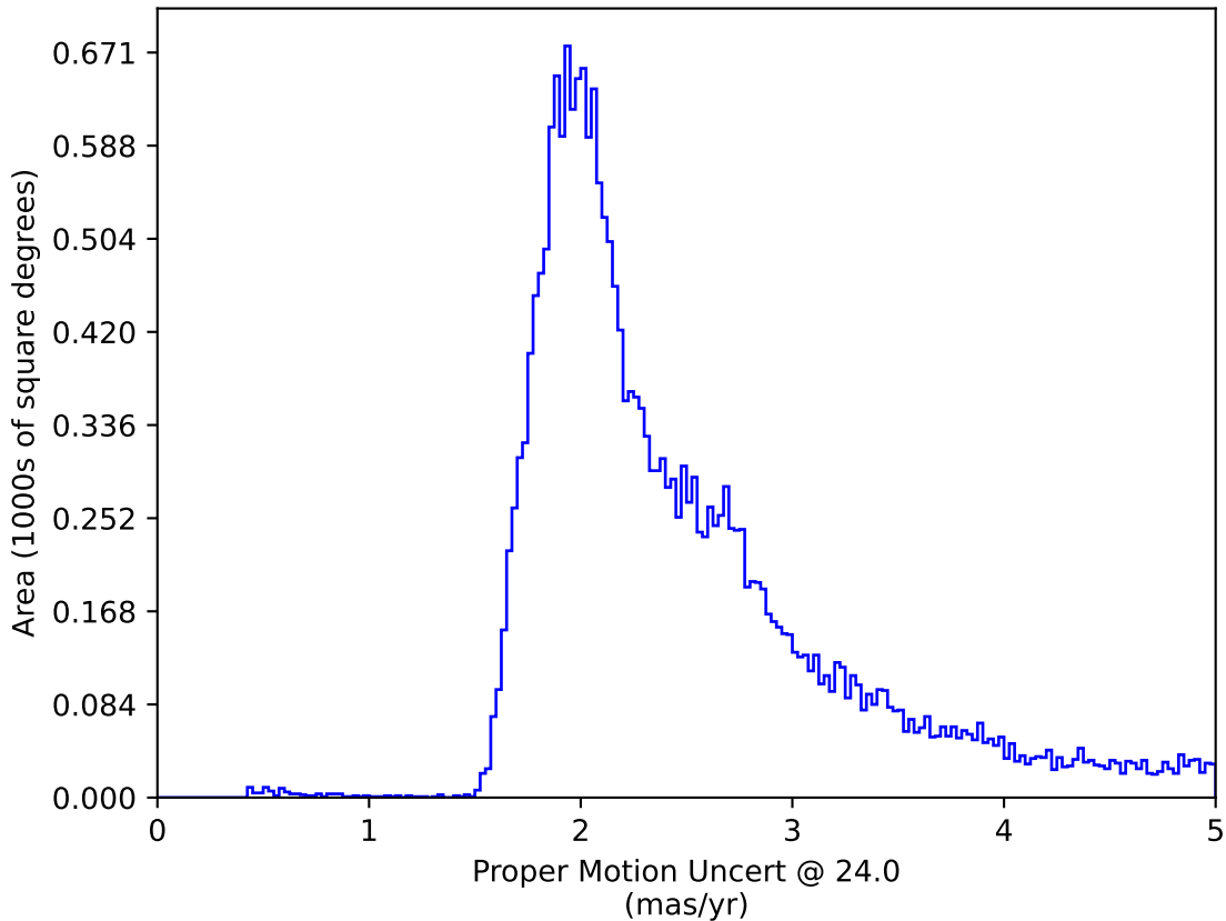
too_elab_r32_d2_giz_v3.4_10yrs : Proper Motion Uncert @ 24.0
