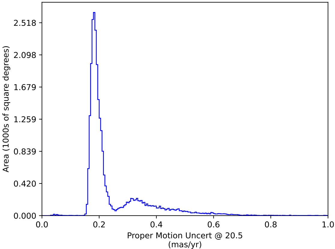
too_elab_r32_d2_giz_v3.4_10yrs : Proper Motion Uncert @ 20.5
